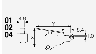
Plain lever
